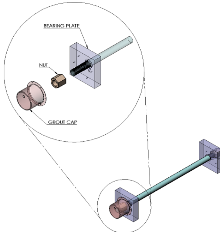
Shear Key's Components
